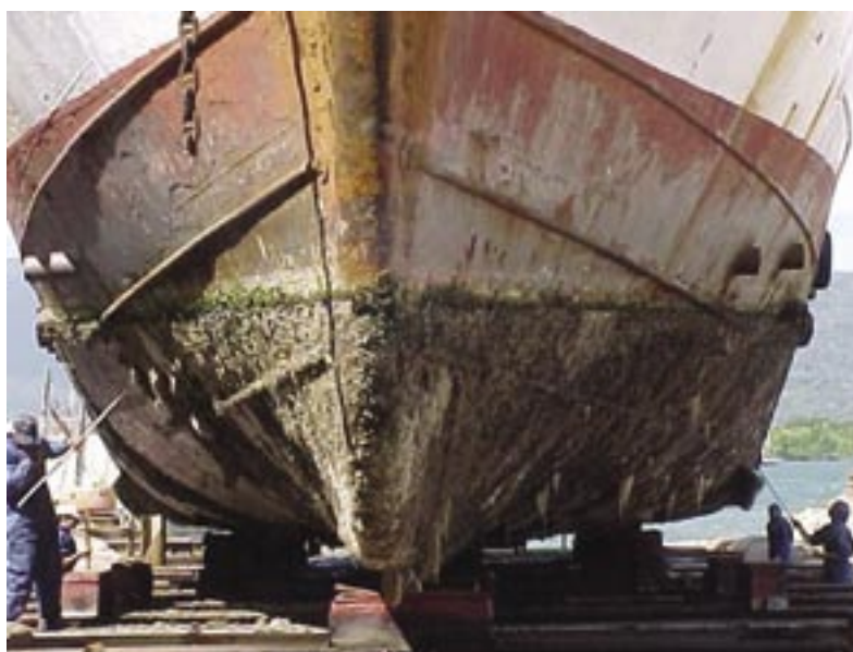
Defouling of an international trading vessel on a Cairns slipway Photo courtesy of Queensland Environment Protection Agency
